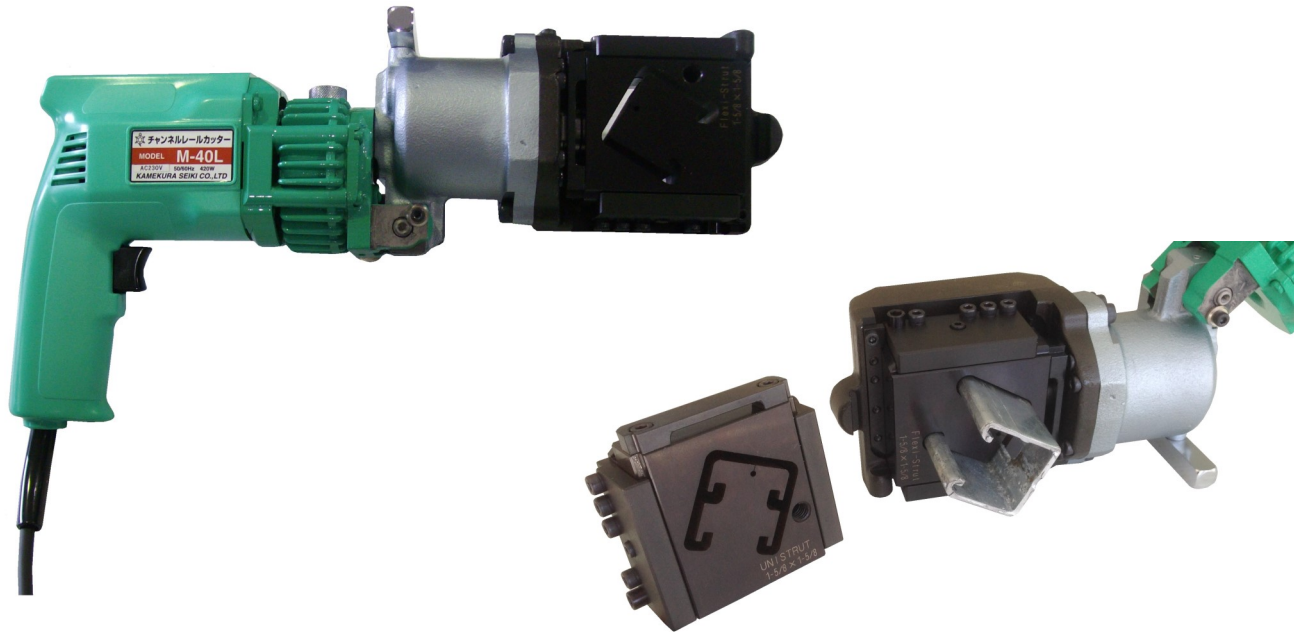
Dual Strut Cutting Profile
